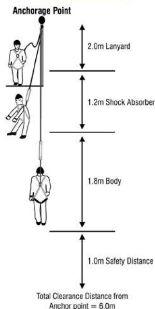
Energy Absorber Ref. PN 300
